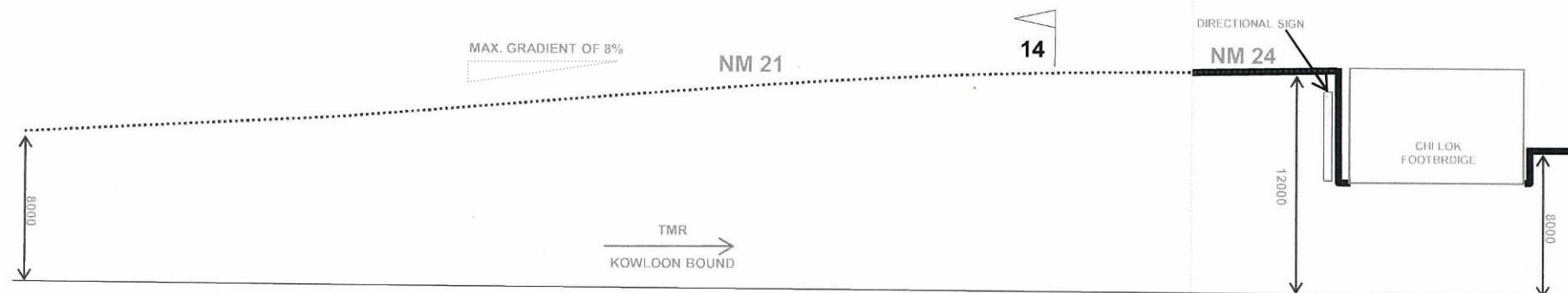
LONGITUDINAL SECTION ALONG TMR KOWLOON BOUND BETWEEN NM21 – NM24 (N.T.S.)
